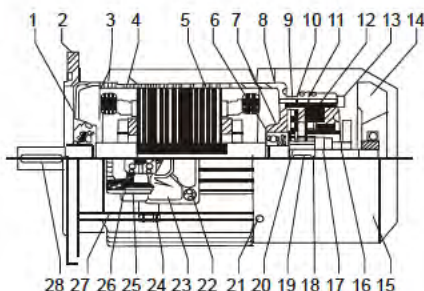
MSEJ Brake Motors B3 132~160
